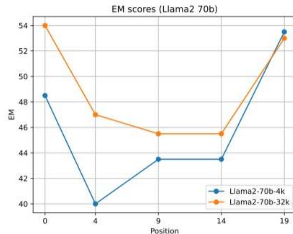
Figure 1: Llama2-70B also displays lost-in-the-middle phenomenon
